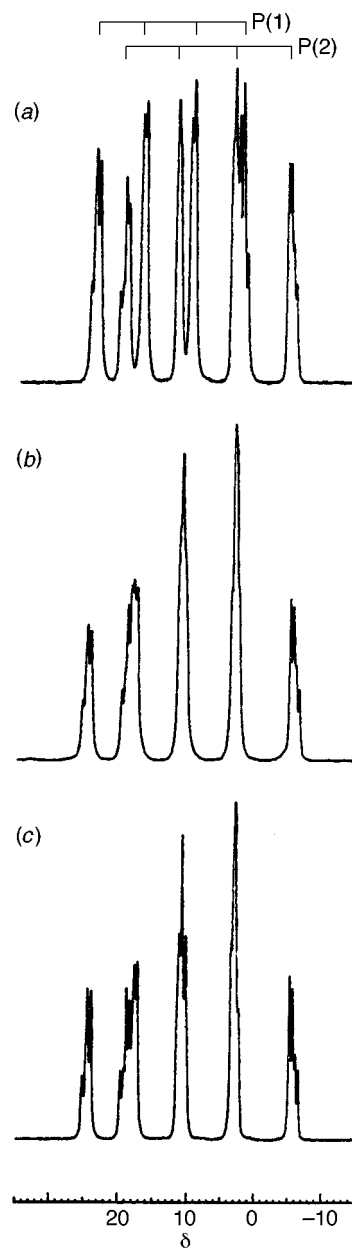
Fig. 3 One-dimensional 31 P CP MAS NMR spectra of [Cu(PPh 3 ) 2 (MeCN) 2 ]X at 9.40 T for X = PF 6 (a), BF 4 (b) and ClO 4 (c). Resolution of the outer components of the 65 Cu multiplet is apparent for each quartet
